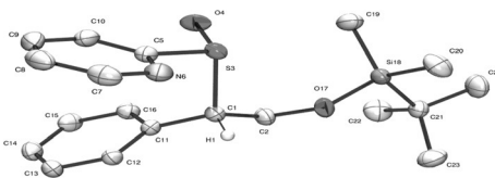
Figure 2. XRD structure of sulfoxide 3ac' (CCDC 1457851). Thermal ellipsoids shown at 50% probability.
